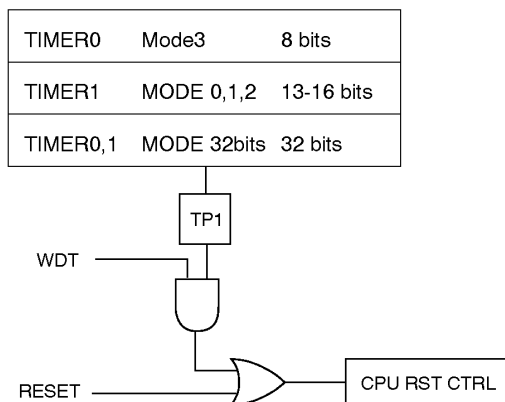
Figure 15. The Different Watchdog Configurations.
