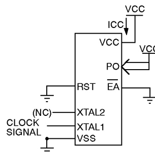
Figure 17. ICC Test Condition, Active Mode. All other pins are disconnected.
