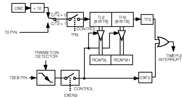
Figure 8. Timer 2 in Auto-Reload Mode.
