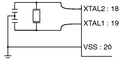
Figure 5. Crystal Oscillator.
