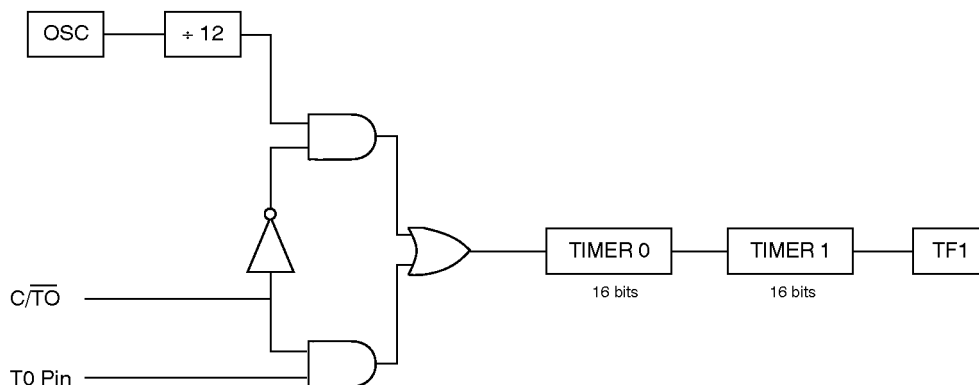
Figure 11. 32 Bit Timer/counter.
