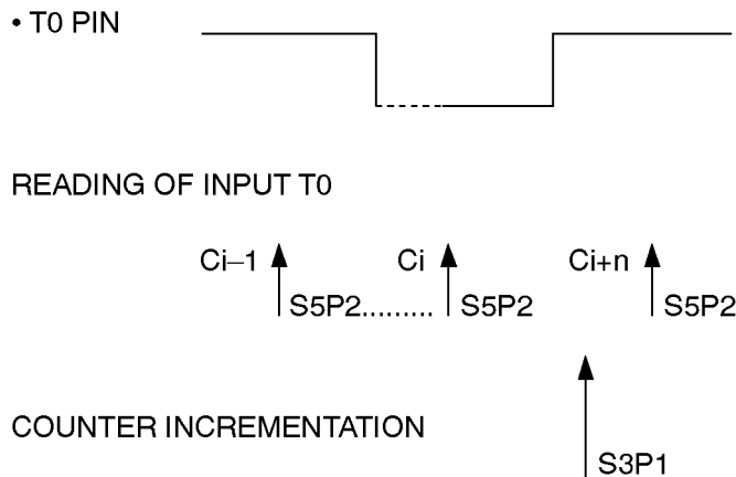
Figure 14. Counter Incrementation Condition.
