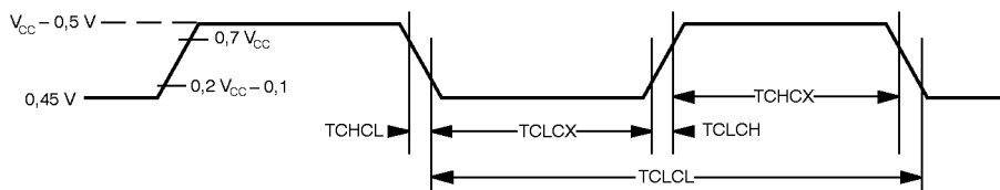
Figure 19. Clock Signal Waveform for ICC Tests in Active and Idle Modes. TCLCH = TCHCL = 5 ns.
